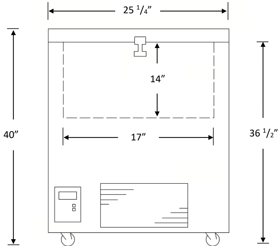
Chest Freezer Front View
